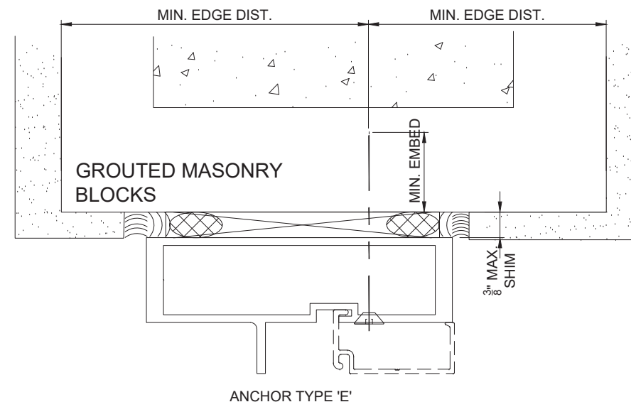
ANCHOR SUBSTRATE OPTIONS WITH DIFFERENT ANCHOR LOCATION OPTIONS
